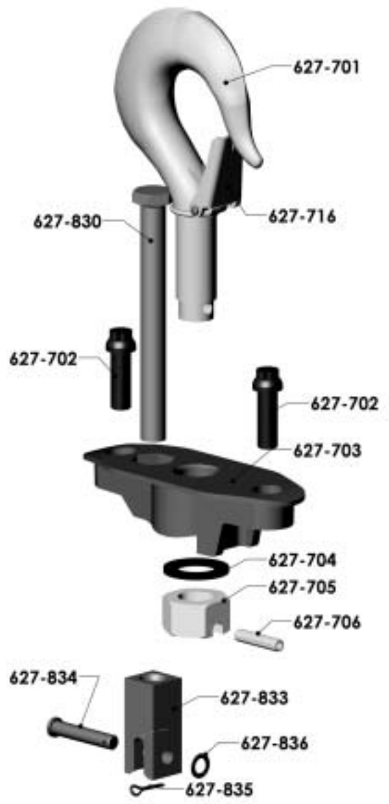
627-700 COMPLETE SWIVEL HOOK SUSPENSION
